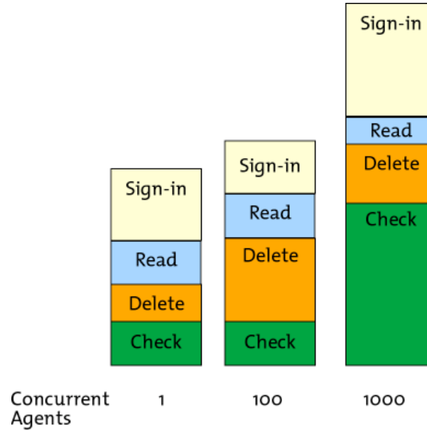
Figure 8-2 Horizontal scalability tests a system's ability to handle increasing levels of load. Notice that the parts of a transaction perform differently under different levels of load.
