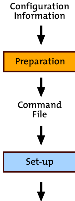
Figure 8-5: A command protocol is shared between the preparation and set-up stages to establish state prior to testing a stateful system.
