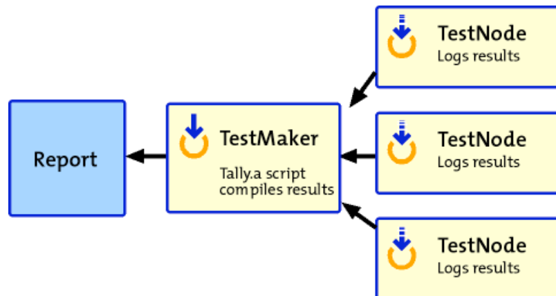
Figure 15-9 While the test runs the test agent scripts logs results data to a log file on the local TestNode machine. At the conclusion of the test the TestNodes return their logged data to the central TestMaker console for analysis and reporting.
