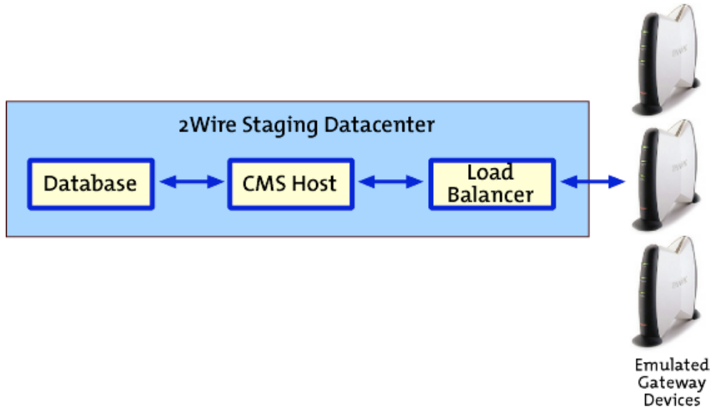
Figure 13-7 A scalability testing configuration checks the CMS datacenter for throughput by increasing the numbers of emulated HomePortal gateway devices.
