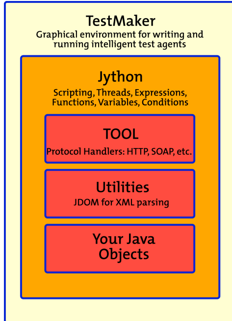
Figure 6-4 An architectural view of the TestMaker environment showing all the components provided to build intelligent test agents.
