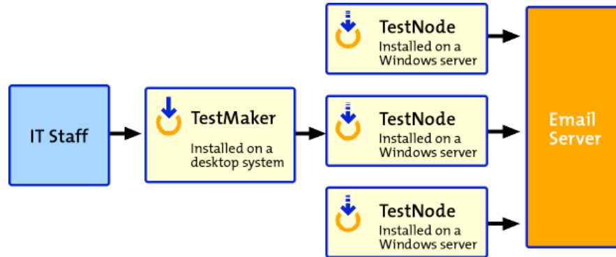
Figure 15-1 The email system test uses TestMaker as a central console to drive the test agents running in several TestNodes. The TestNodes for this test are inexpensive Intel-based Windows servers running the TestNetwork software. The test agents emulate virtual users to drive load on the email server.
