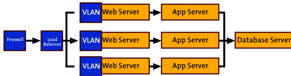
Fig. 10-5: Load balancers are dynamic routers that assign and manage affinity from user machines to a host for the duration of a user session.
