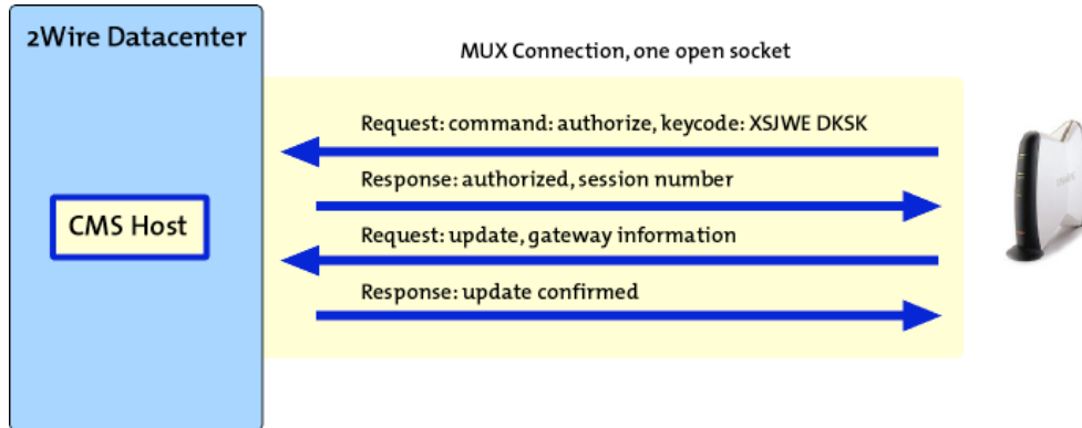
Figure 13-3 To more efficiently use network sockets, the 2Wire CMS protocol uses a MUX layer. The gateway box opens a socket and both the gateway and the server make requests over the open socket.
